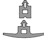
CAM TABLOSU / GLAZING BEAD (CE2-03)/(CE2-04)
